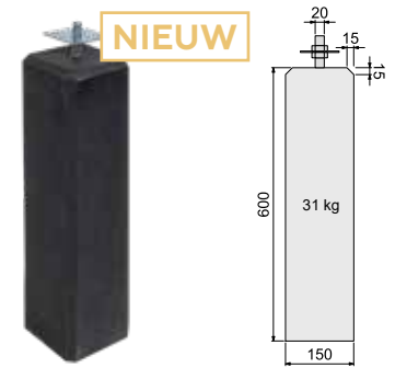
Betonpoer antraciet
