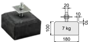
Betontegel antraciet
